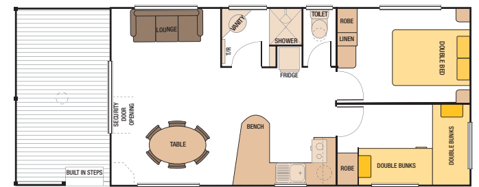
38' x 15' - No.1 Cabin (11582mm x 4570mm) Code: 38P1004
