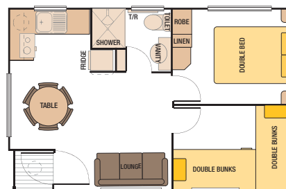
23'6" x 15' - No.2 Cabin (7160mm x 4570mm) Code: 236P1002
