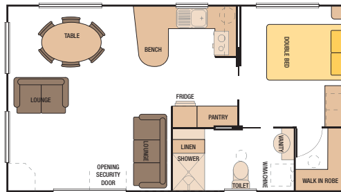
28' x 15'5' - No.3 Cabin (8534mm x 4700mm) Code: 28P1003
