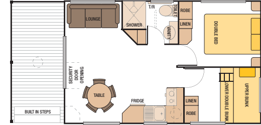
29' x 14' - No.3 Cabin (8840mm x 4300mm) Code: 29P1003
