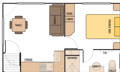
22' x 13' - No.1 Cabin (6706mm x 3962mm) Code: 22P1001
