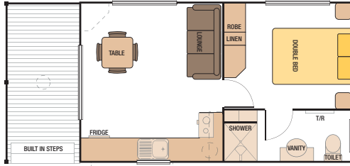
28' x 13' - No.1 Cabin (8534mm x 3962mm) Code: 28P1001
