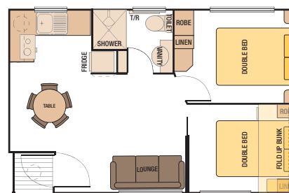
23'6" x 15' - No.1 Cabin (7160mm x 4570mm) Code: 236P1001
