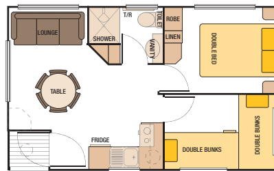
23' x 14' - No.2 Cabin (7010mm x 4300mm) Code: 23P1002
