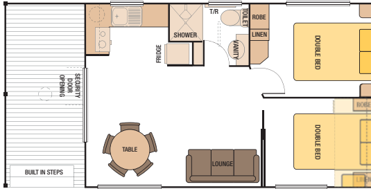
30' x 15' - No.1 Cabin (9144mm x 4570mm) Code: 30P1001
