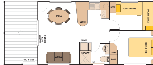
36' x 15'5" - No.2 Cabin (11000mm x 4700mm) Code: 36P1002
