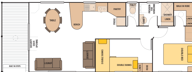
42' x 15'5" - No.1 Cabin (12800mm x 4700mm) Code: 42P1001
