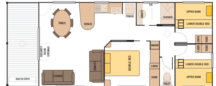
38' x 15'5" - No.3 Cabin (11582mm x 4700mm) Code: 38P1002
