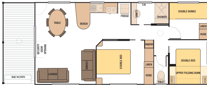
39' x 15'5" - No.1 Cabin (11887mm x 4700mm) Code: 39P1002
