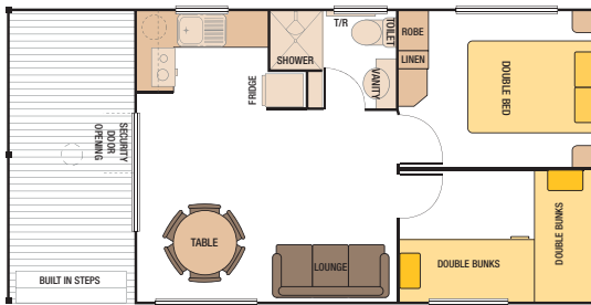
30' x 15' - No.2 Cabin (9144mm x 4570mm) Code: 30P1002
