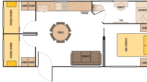
29' x 14' - No.4 Cabin (8840mm x 4300mm) Code: 29P1002
