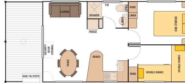
34' x 15' - No.1 Cabin (10350mm x 4570mm) Code: 34P1002
