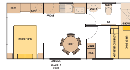
25' x 11' - No.1 Cabin (7620mm x 3352mm) Code: 25P1002
