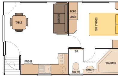
23' x 14' - Spa No.1 Cabin (7010mm x 4300mm) Code: 23P1004
