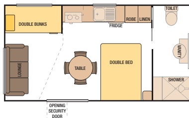
21' x 11' - No.1 Cabin (6400mm x 3352mm) Code: 21P1001
