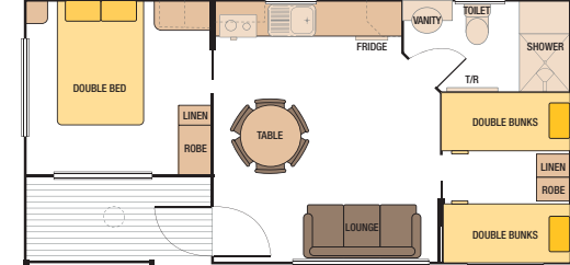
29' x 14' - No.2 Cabin (8840mm x 4300mm) Code: 29P1004
