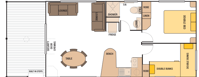
38' x 15'5" - No.2 Cabin (11582mm x 4700mm) Code: 38P1001
