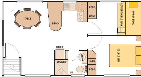
28' x 15' - No.2 Cabin (8535mm x 4570mm) Code: 28P1002
