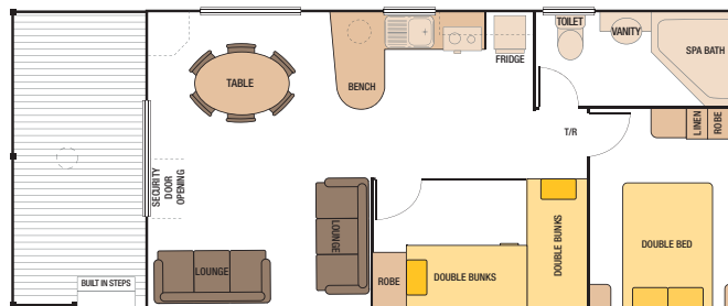
38' x 15'5" - Spa No.3 Cabin (11582mm x 4700mm) Code: 38P1003
