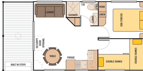
29' x 14' - No.4 Cabin (8840mm x 4300mm) Code: 29P1002
