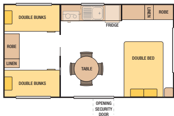
20' x 11' - No.1 Cabin (6096mm x 3206mm) Code: 20P1001
