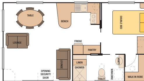
28' x 15'5' - No.3 Cabin (8534mm x 4700mm) Code: 28P1003
