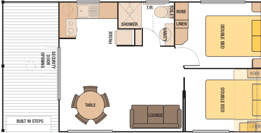
30' x 15' - No.1 Cabin (9144mm x 4570mm) Code: 30P1001
