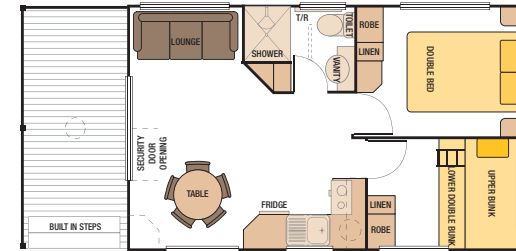
29' x 14' - No.3 Cabin (8840mm x 4300mm) Code: 29P1003
